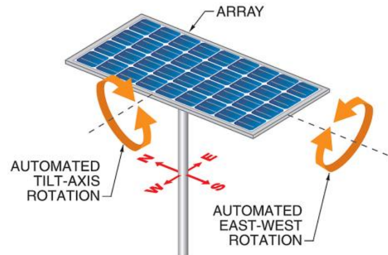
EQUATORIAL TRACKING
